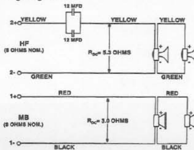
FIGURE 7 — Wiring Diagram
